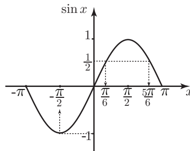
Figure 1. A graph of \sin x over the interval -\pi \leq x < \pi .
